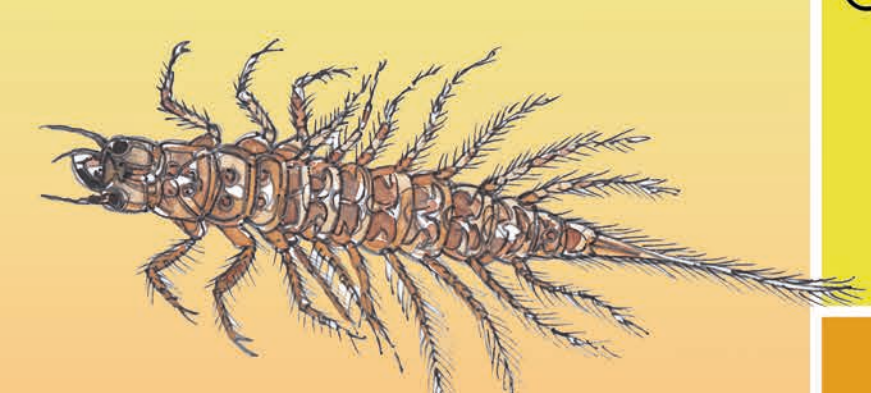
Schlammfliegenlarve 20-40 mm
