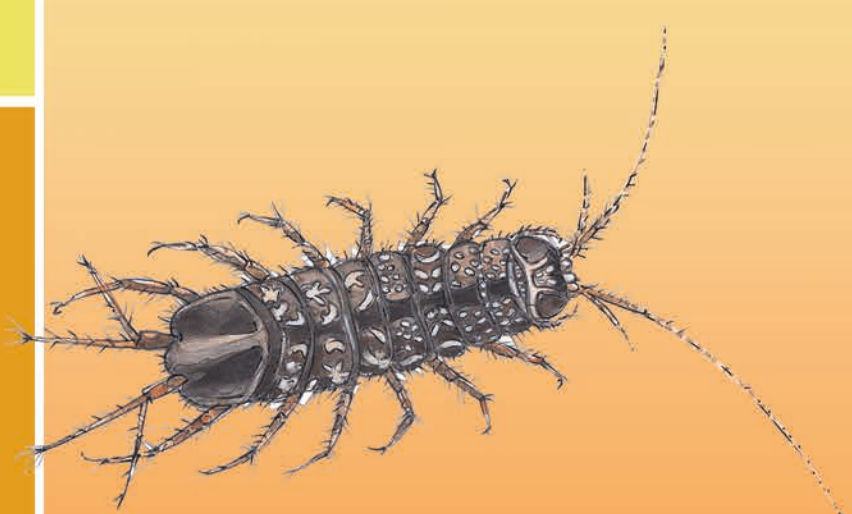
Wasserassel 12 mm
